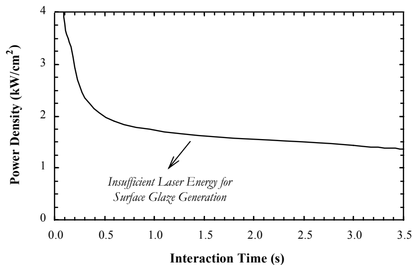
Figure 2. Relationship between laser power density and glazing interaction time on concrete for the 2.5 kW HPDL.
