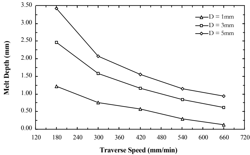
Figure 8. Effect of aperture size ( D ) on the maximum melt depth for OPC with increasing traverse speed.
