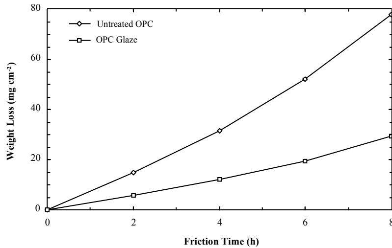
Figure 6. Relationship between weight loss and friction time for the laser generated glaze and the untreated OPC.
