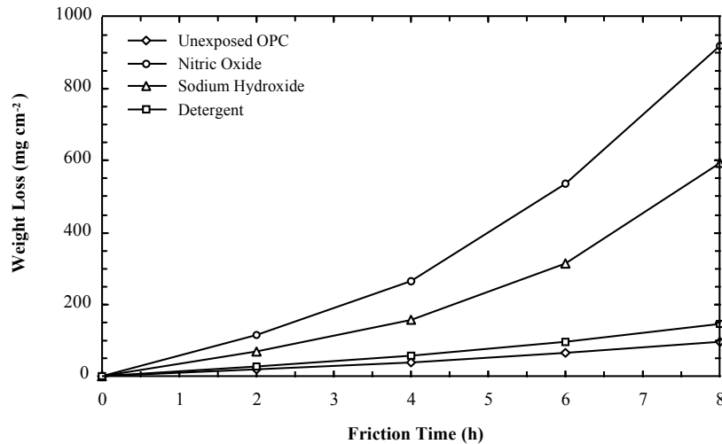
Figure 7. Relationship between weight loss and friction time for the untreated OPC with different reagent types at the maximum concentration (80%).
