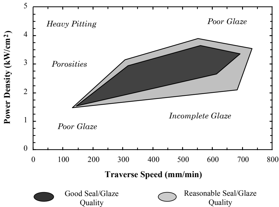
Figure 3. Schematic representation of the operating window for the concrete glazing process using the 2.5 kW HPDL.
