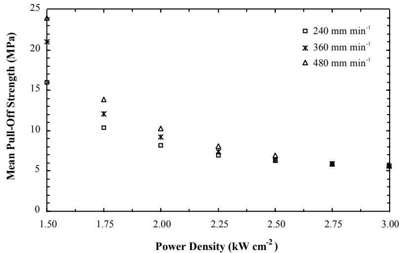
Figure 4. Relationship between pull-off strength of laser glaze with laser power density.
