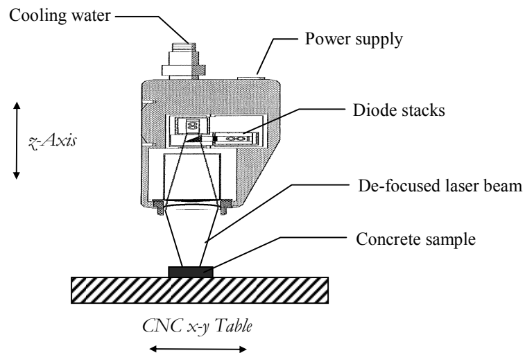
Figure 1 . Schematic representation of the 2.5 kW HPDL head assembly.
