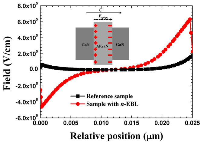
FIG. 6. Electric field profiles in the region of the n -EBL layer for the Sample with n -EBL and the GaN layer for the Reference. Inset shows the polarized GaN/AlGaN/GaN heterostructure. The positive direction of the electric field is along the growth orientation, i.e., c+ orientation. The data are collected at the current level of 25 \text{ A/cm}^2 .
