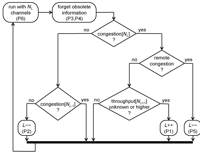
Fig. 2. High-level description of the control algorithm.
