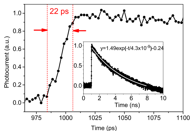
FIG. 5. Rise time of the device. (Inset) Time response in nanosecond scale.
