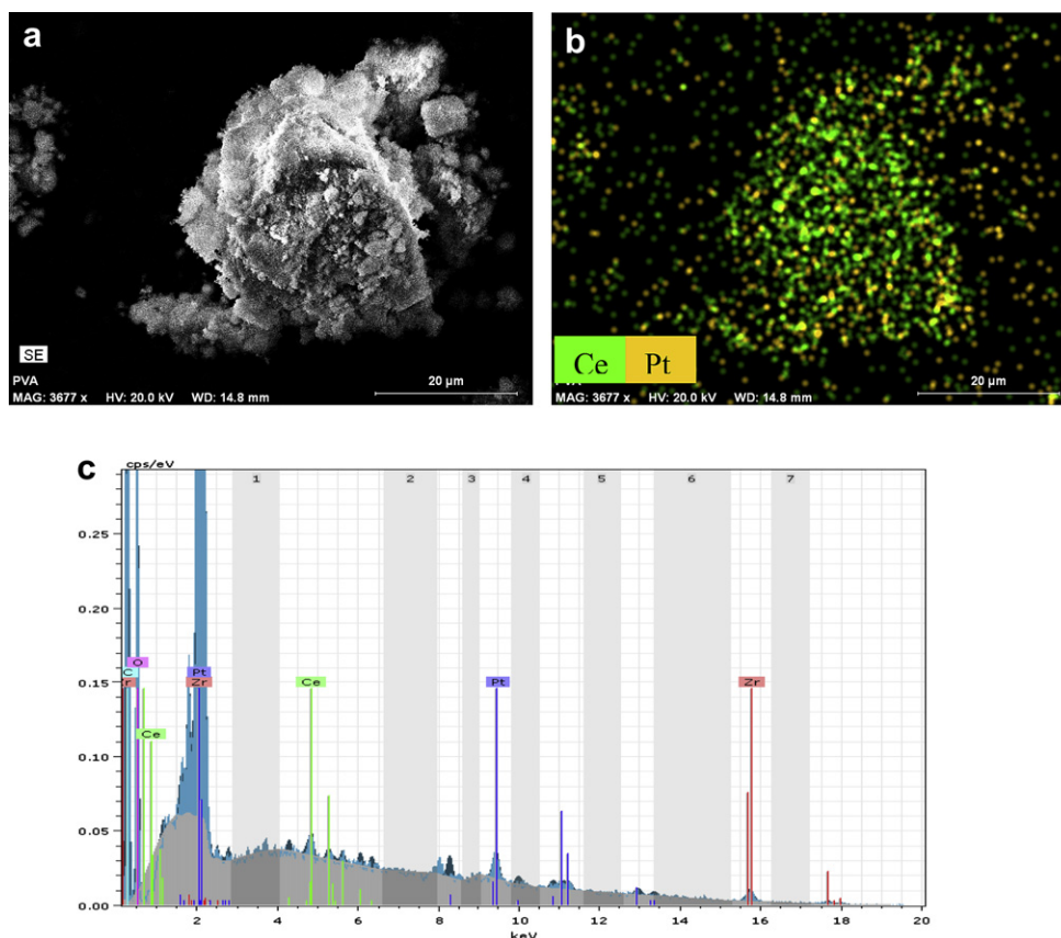
Fig. 5 – 1%Pt–1%Ce/ZrO 2 catalyst prepared by seq. impregnation (cat4): (a) SEM bright area image, (b) Pt + Ce mapping, and (c) EDX spectrum.
