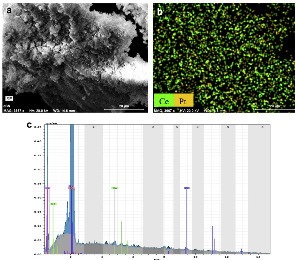
Fig. 4 – 1%Pt-1%Ce/ZrO 2 catalyst prepared by coimpregnation (cat2): (a) SEM bright area image, (b) Pt + Ce mapping, and (c) EDX spectrum.
