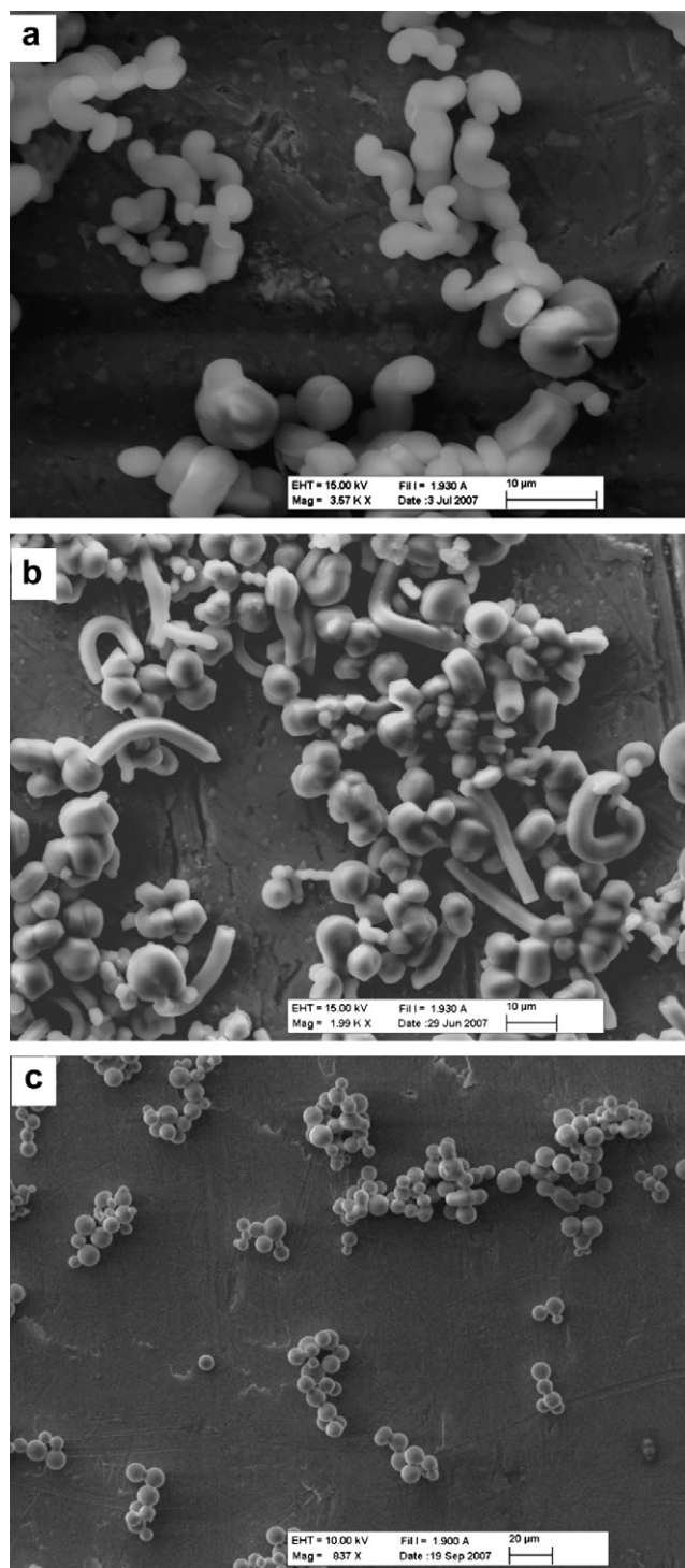
Fig. 6. The SEM images of mesostructured silica obtained from CTAB–P85 system with a CTAB/P85 mole ratio of 2.50 in the presence of (a) 1 g KCl, (b) 5 ml Cyclohexane, and (c) 1 g NaNO 3 .
