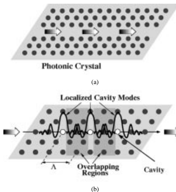
Fig. 1. Schematic drawing of two different waveguiding mechanisms in photonic crystals. (a) Planar waveguides (PW) consist of two parallel photonic crystal mirrors with a suitable separation between them. Photons propagate through the opening which can be considered a continuous defect. (b) CCWs are formed by removing an array of rods (white circles) from a 2-D photonic crystal (black circles). Tightly confined cavity mode interacts weakly with the neighboring cavity modes, and therefore the electromagnetic waves can propagate through coupled cavities.
