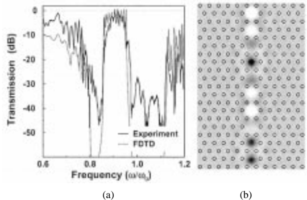
Fig. 4. (a) Measured (solid line) and calculated (dotted line) transmission spectra of the straight CCW which is generated by removing 10 adjacent rods from the crystal. A cavity band is formed extending from 0.857 \omega_0 to 0.956 \omega_0 . Nearly 100% transmission is achieved for certain frequencies. (b) Calculated field distribution of the CCW for a frequency within the cavity band, namely, \omega = 0.920 \omega_0 . The guided mode travels along the cavities due to coupling between the localized cavity modes. The electric field \mathbf{E} is polarized along the axis of missing rod.
