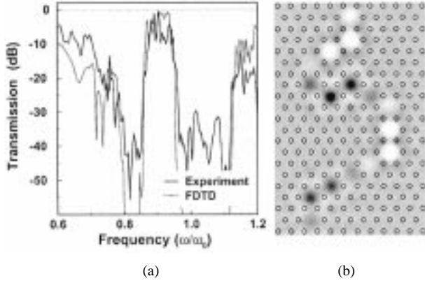
Fig. 5. (a) Measured (solid line) and calculated (dotted line) transmission spectra of the zig-zag CCW which contains 16 cavities. (b) Calculated field distribution of the zig-zag CCW for a frequency within the cavity band, namely, \omega = 0.936 \omega_0 .
