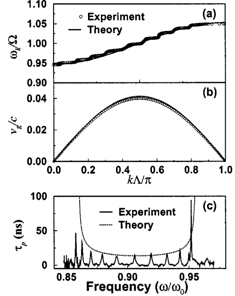
Fig. 6. Comparison of the measured and calculated: (a) dispersion relation; (b) group velocity; and (c) delay time corresponding to the straight CCW. Equations (9), (11), and (13) are used to determine \omega(k) , v_g , and \tau_p with \kappa = -0.0525 , respectively. There is good agreement between the experimental results and the predictions of the tight-binding approximation.
