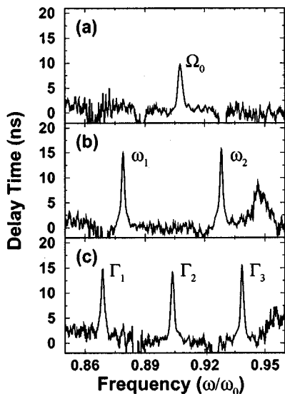
Fig. 3. Measured delay time characteristics of the corresponding coupled-cavity structures, namely: (a) single cavity; (b) two coupled-cavity; and (c) three coupled-cavity. \tau_p exhibit peaks at the resonance frequencies which implies that photons spend more time inside the cavities for these frequencies.
