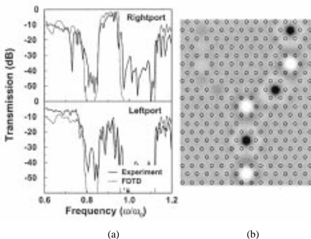
Fig. 8. (a) Measured (solid line) and calculated (dotted line) transmission characteristics of a coupled-cavity switching structure. (b) Corresponding field pattern clearly indicates that most of the power is coupled to the right port.
