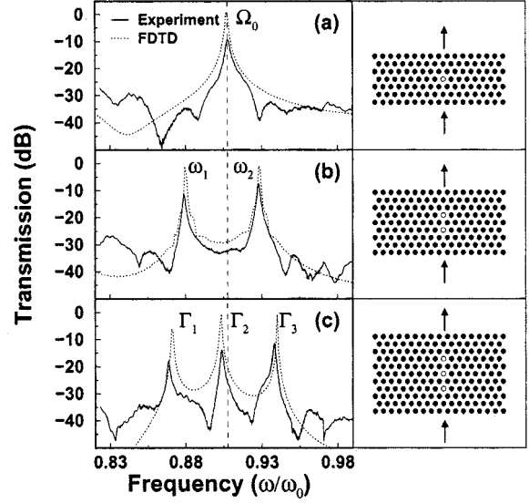
Fig. 2. Left panels: Measured (solid lines) and calculated (dotted lines) transmission spectra by using FDTD method for: (a) a single cavity; (b) two coupled-cavity; and (c) three coupled-cavity structures. Due to coupling between the strongly localized cavity modes, single cavity mode splits into two or three distinct modes depending on the number of coupled cavities. There is good agreement between the measured and calculated transmission spectra. Right panels: Schematics of the corresponding coupled-cavity structures where (o) symbols denote the removed rods.
