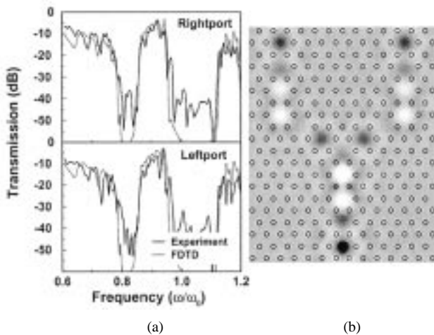
Fig. 7. (a) Measured (solid line) and calculated (dotted line) of transmission spectra of a Y-shaped coupled-cavity based splitter. The electromagnetic power in the input port splits equally into the two output waveguide ports for frequencies throughout the cavity band. (b) Calculated power distribution inside the input and the output waveguide channels of the splitter for frequency \omega = 0.916 \omega_0 .
