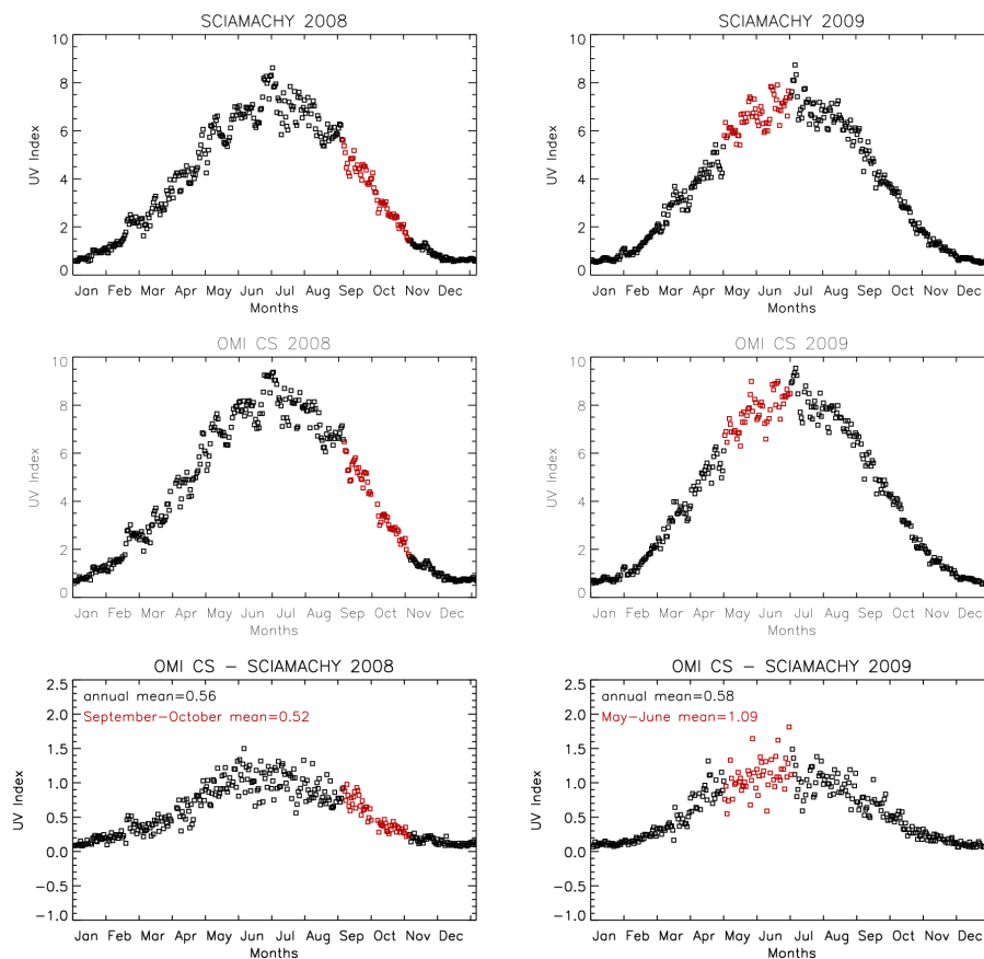
Fig. 2. SCIAMACHY and OMI (clear-sky data) satellite 2008 (left) and 2009 (right) UVI products. Bottom figures: absolute mean difference between OMI clear sky and SCIAMACHY products for 2008 (left) and 2009 (right). Red squares: RISC UV campaign periods.
