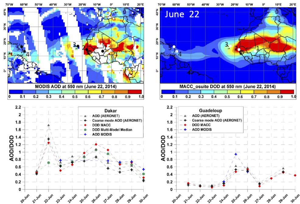
Figure 2. (Top) daily averaged DOD from MACC o-suite (top right, with the AERONET sites marked with white dots: 1 – IER Cinzana; 2 – Dakar; 3 – Capo Verde; 4 – Barbados; 5 – Guadeloup) and daily AOD from MODIS-AQUA (AOD Ocean + DeepBlue) (top left, with the AERONET sites marked with black dots) for 22 June 2014. (Bottom) coarse mode AOD at 500 nm (DOD) (black crosses) and AOD at 550 nm (grey triangles) from AERONET, DOD from MACC o-suite (red diamonds), and AOD retrieved from MODIS-AQUA (blue crosses) at Dakar and Guadeloup AERONET sites during the case analysis from 21 to 30 June 2014.
