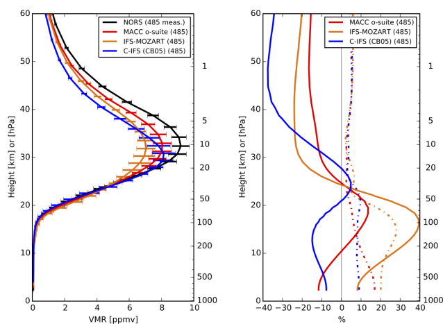
Figure 9. Comparison of the average O_3 mixing ratios of MACC o-suite (red), IFS–MOZART (orange) and C-IFS (CB05) (blue) with the average NDACC FTIR profiles (black) observed at Izaña ( 28.3^\circ N , 16.5^\circ W ) for the period September 2013–September 2014. (Left) O_3 profiles, (right) profiles of the bias and standard deviation of the differences centred on the bias. The number of available O_3 profiles and the number of collocated model profiles are indicated in between brackets.
