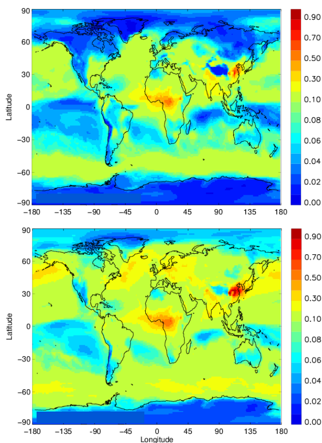
Figure 1. E-suite verification example. Total AOD plots showed that there was a considerable loss of aerosol of 30 %, from a mean AOD of 0.14 to 0.094, after a 96 h forecast in the e-suite (top panel) compared to the o-suite (bottom panel). The Ångström exponent showed considerably smaller particles in the e-suite as compared to the o-suite. Because of this the o-suite upgrade of April 2013 was postponed. The problem was solved and a new e-suite run was tested positively in August 2013. Example taken from the e-suite report of April 2013 (Eskes et al., 2013).
