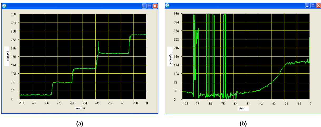
Figure 2: Location results in (a) semi-anechoic chamber and (b) open space
