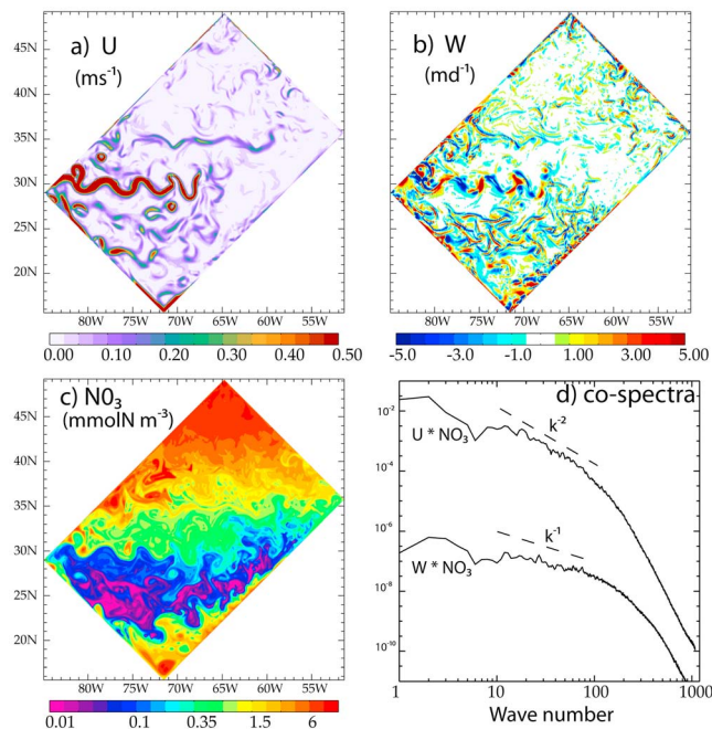
Figure 3. Snapshots of (a) modulus of horizontal velocity ( U ), (b) vertical velocity ( W ) and (c) nitrate concentration ( \text{NO}_3 , in log scale) from an idealized submesoscale-resolving model simulation representative of the Northwest Atlantic or Northwest Pacific subtropical to subpolar regions. Model fields are shown at 50 m depth, in winter (Dec 1st). (d) Co-spectra of U * \text{NO}_3 and W * \text{NO}_3 , plotted in log-log scale.
