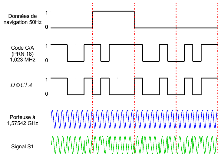
Figure 2.4 — Structure d'un signal GPS
