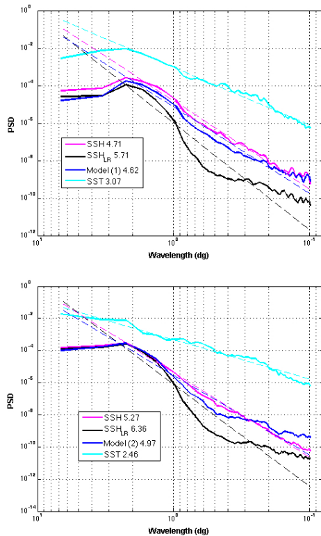
FIGURE 4: Spectral analysis of the results reported in Fig. 2 and 3 : we report the radially-averaged power spectral densities of the different fields for February 10, 2010 (top) and August, 8, 2010 (bottom).
