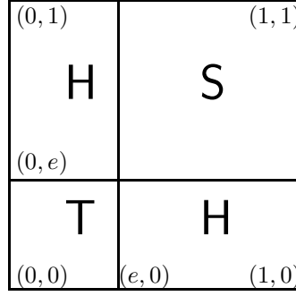
Figure 2: The representation of a uninorm from Proposition 19
