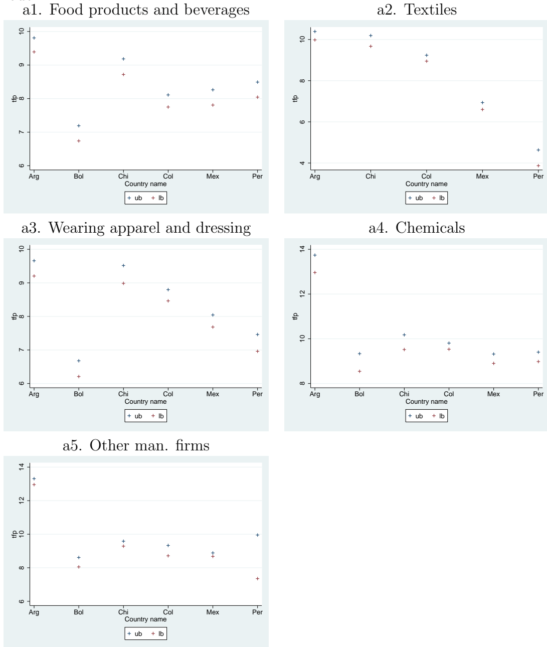
Figure 10: Sub-sectors: average TFP confidence interval by country, baseline model
