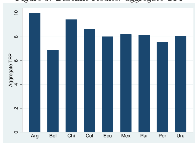
Figure 3: Baseline results: aggregate TFP
