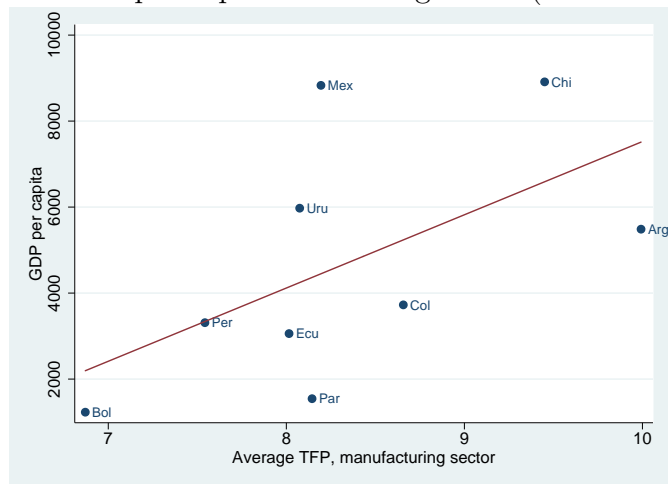
Figure 2: GDP per capita and average TFP (baseline results)
