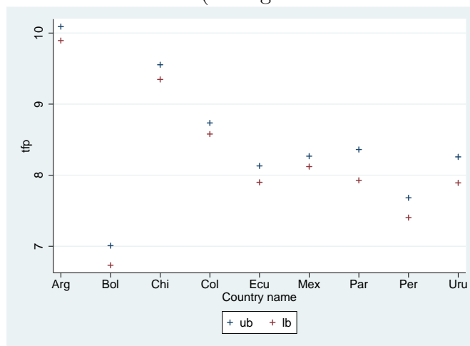
Figure 1: Baseline results (average TFP confidence intervals)
