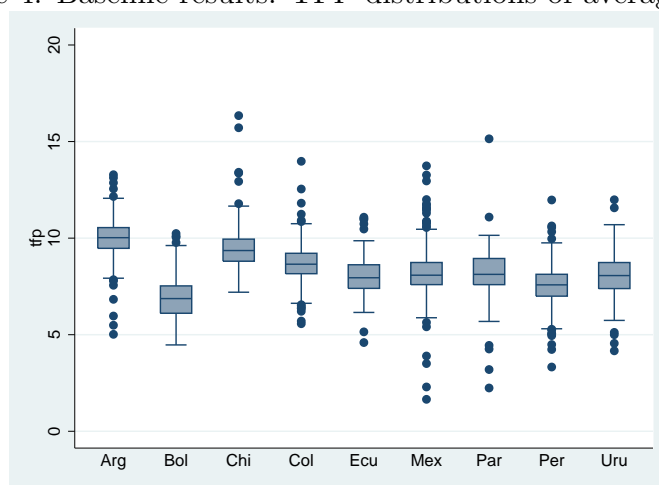
Figure 4: Baseline results: TFP distributions of average TFP
