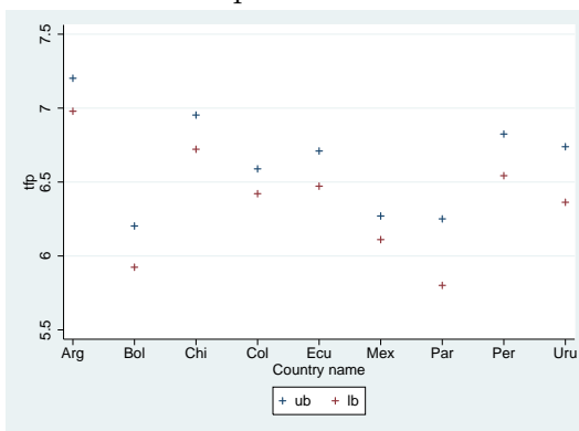
Figure 9: Comparing different specifications: average TFP confidence interval by country (factor elasticities constant across countries)
