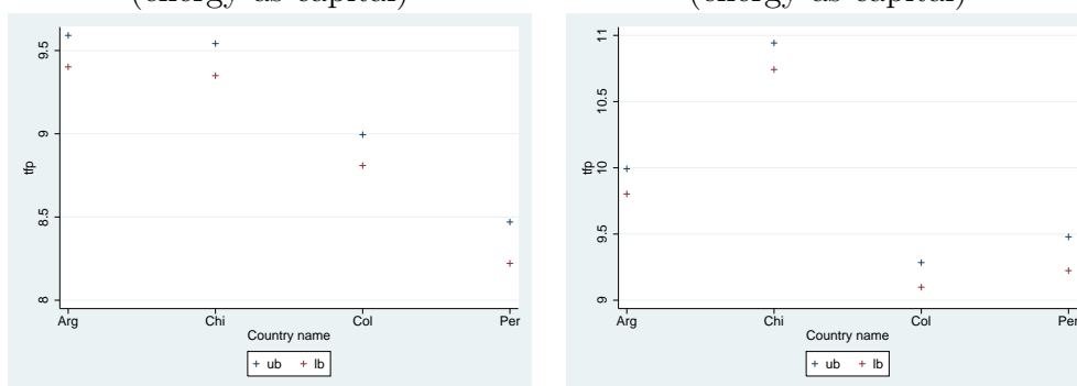
Figure 12: Panel results: average TFP confidence interval by country a. Pooled OLS b. Fixed Effects (energy as capital)
