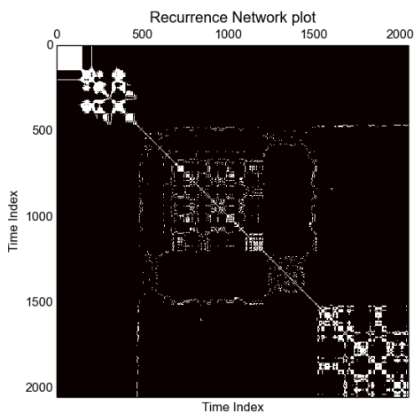
(c) Recurrence plot of adjacency.
