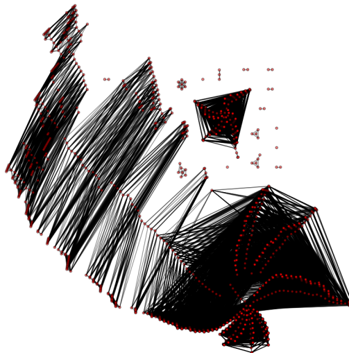
(d) Recurrence network with the Internet lanl Routes representation
