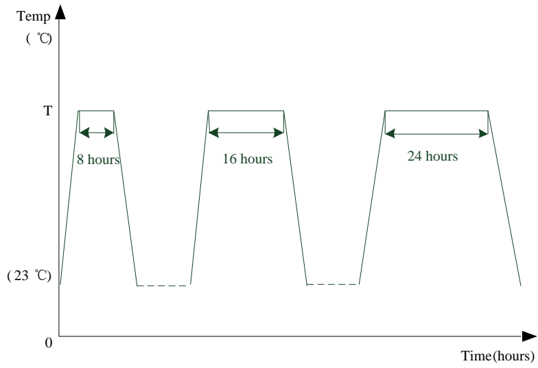
Figure 7. ADT profile
