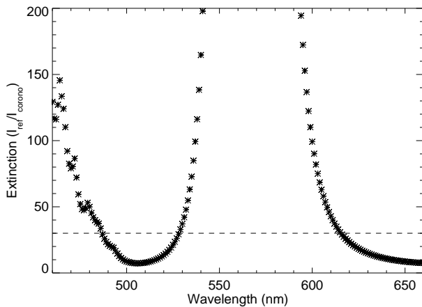
Fig. 5. Curve showing the wavelength-dependent extinction ( \max(I_{\text{reference}}) / \max(I_{\text{coronagraph}}) ) (stars) due to the refractor focus chromatism and the extinction limit (dashed line) for the whole spectrum (polychromatic coronagraphic image), which only reaches \sim 30 . The vertical scale has been truncated (because the pure performance would be limited by the component itself to approximately 1000). A spectral filter would clearly increase the extinction limit potential between 550 nm and 590 nm.
