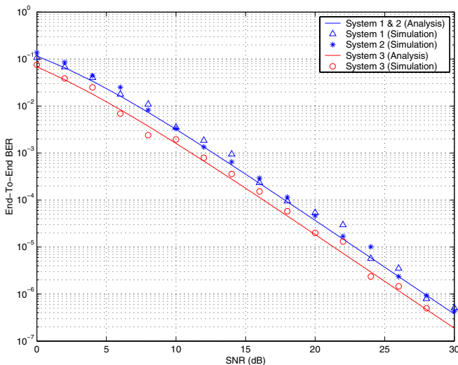
Fig. 5. Comparison between end-to-end bit-error rate of the three configurations.
