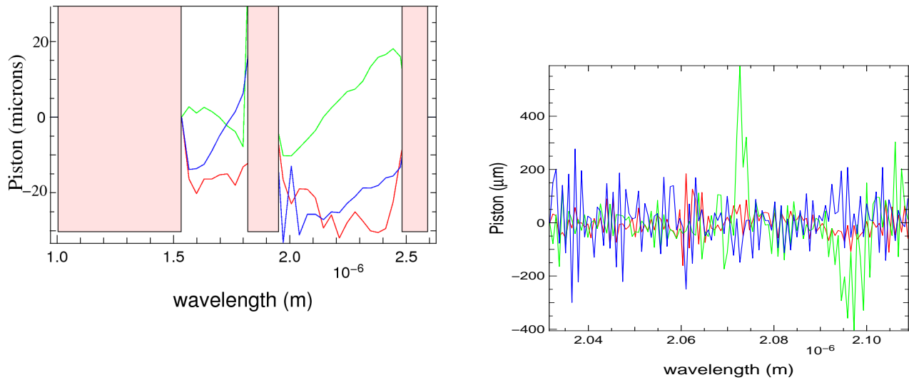
Figure 2. Left : Example of a non-zero OPD on a P2VM. The masked zones correspond to the inter-bands and the J band where the OPD cannot be computed. Right : Example of a \gamma^2 Vel observation, where the object’s phase can introduce chromatic “OPD” as high as 500\mu\text{m} , which is no longer negligible for this medium resolution data (same as the one of Fig. 5).
