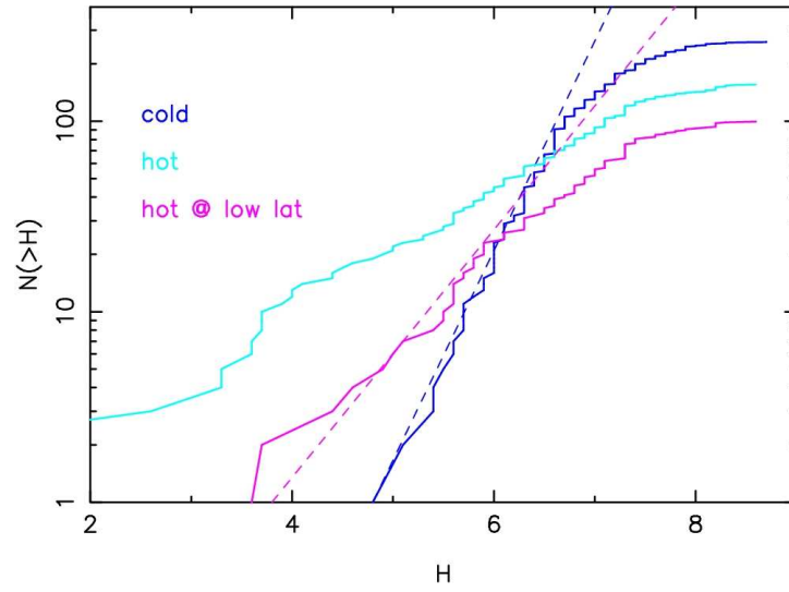
Fig. 2.— The absolute magnitude ( H ) cumulative distributions of the cold population (blue), of the hot population (cyan) and of the objects of the hot population discovered within 4.5^\circ of the ecliptic (magenta). For reference, the thin dashed blue line has a slope of 1.1; the thin dashed magenta line has a slope of 0.65.
