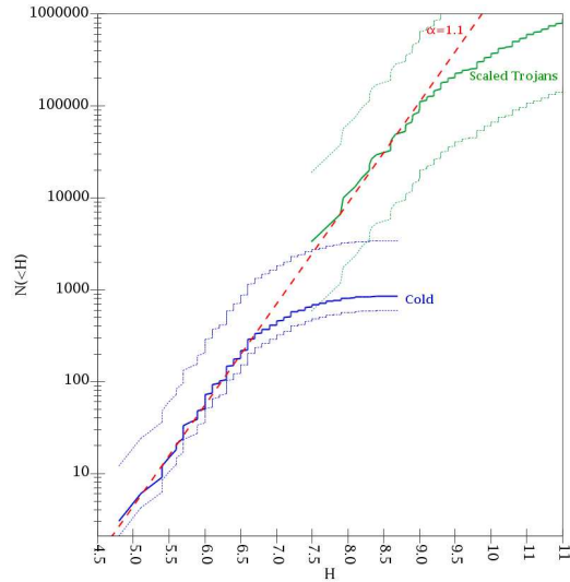
Fig. 3.— The cumulative H -distributions of the cold population (blue lines) and of the Trojan population (green lines). The blue dotted lines bracket the current number of cold KBOs according to B04. The dotted green curves show the current HD of the Trojans, scaled by factors of 600 (lower curve) and 19,000 (upper curve), which correspond to the minimal and maximal ratios between the populations of cold KBOs and Trojans, according to the Nice model. The solid blue and green curves show the observed HDs of the cold KBOs and Trojans, scaled by appropriate factors so that they fall within the boundaries provided by the dotted curves. The red dashed line corresponds to an HD with \alpha = 1.1 . This line highlights that the HD of the Trojan population with H < 9 has the same slope of the HD of the cold population with H < 6.5 . We interpret the apparent turn-over of the HD of the cold population at H = 6.5 as due to observational biases. The common slope of the HDs of cold KBOs and Trojans supports the genetic link between these two populations predicted by the Nice model.
