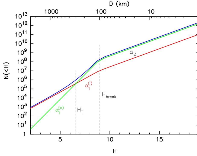
Fig. 1.— Sketch of the HDs in the inner (red) and outer (green) parts of the disk, showing the meaning of the quantities \alpha_1^{(i)} , \alpha_1^{(o)} , \alpha_2 , H_T and H_{\text{break}} . The values of these quantities that we adopt to draw this figure are those that characterize the disk model defined in Sect. 3. The blue curve shows the HD obtained summing the HDs for the inner and the outer parts of the disk. We expect that the current HDs of the cold and of the hot populations of the Kuiper belt have the same shapes of the green and of the blue curves, respectively. The HD of the Trojans has the shape of the blue curve, but is defined only for H > 7.5 (the absolute magnitude of the brightest Trojan). The correspondence between the size scale (top) and H scale (bottom) has been obtained assuming a 4.5% albedo. For simplicity, we assume that the albedo is size-independent.
