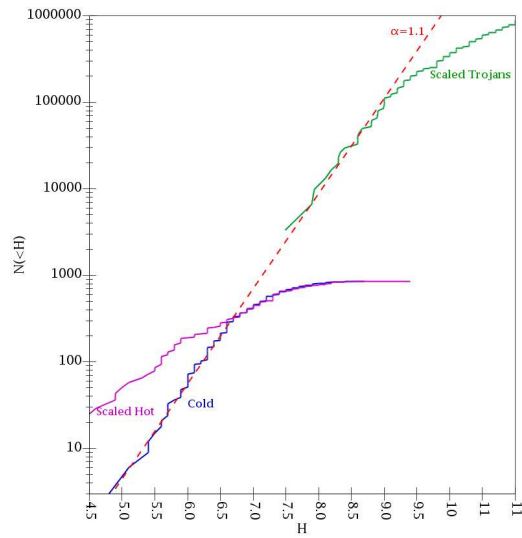
Fig. 4.— The same as Fig. 2, but only the solid curves for the cold KBOs and Trojans are plotted, while the HD of the hot population has been added, scaled up by a factor of 2.5. Notice that the observed HDs of the cold and of the hot populations are identical for H > 6.5 , in agreement with our predictions. See text for a broader discussion on this point.
