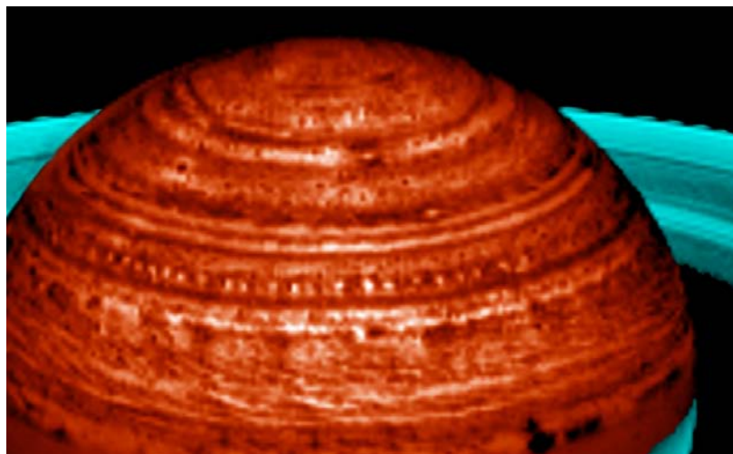
Figure 4: Infrared image taken by the Cassini VIMS instrument in the 5 \mu\text{m} band of the northern hemisphere of Saturn, showing zonal bands and various waves and eddies (such as the 'string of pearls' around 40^\circ\text{N} ), representing features located in the vertical around pressure levels of 1-3 bars.
