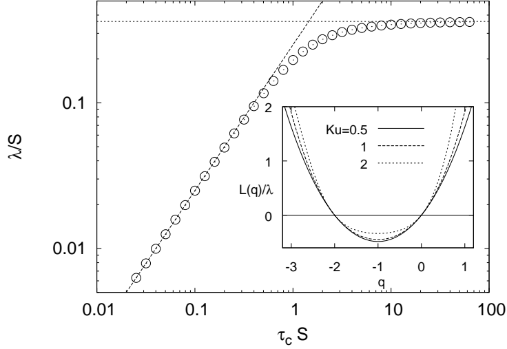
FIGURE 1. Lyapunov exponent as a function of \tau_c (circles). Dashed and dotted lines represent the asymptotic behaviours (3.5) for \tau_c \rightarrow 0 and \tau_c \rightarrow \infty , respectively. Inset: Generalized Lyapunov exponents L(q) for three values of Ku . Note that L(-d) = L(0) = 0 in agreement with the properties of the generalized Lyapunov exponents proved by Zel'dovich et al. (1984).
