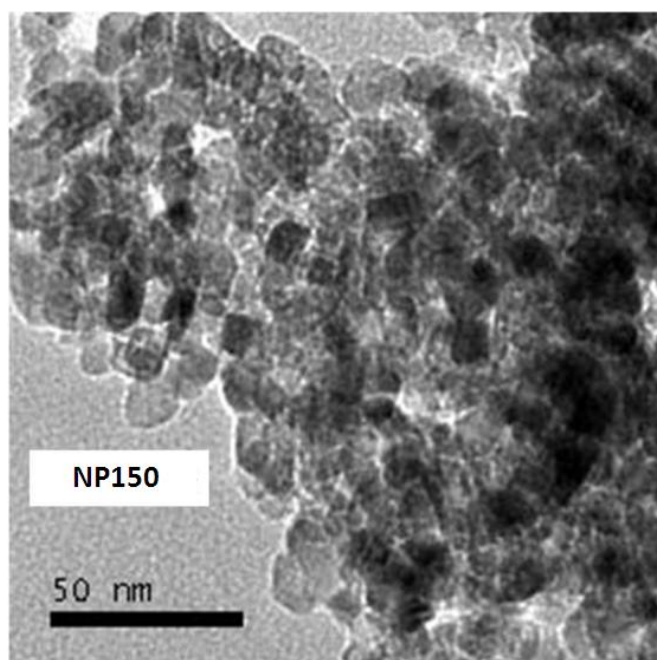
Fig. 3. TEM picture of the nanoparticles NP 150, calcined at T = 150 °C, from the alkaline suspension (pH=10).
