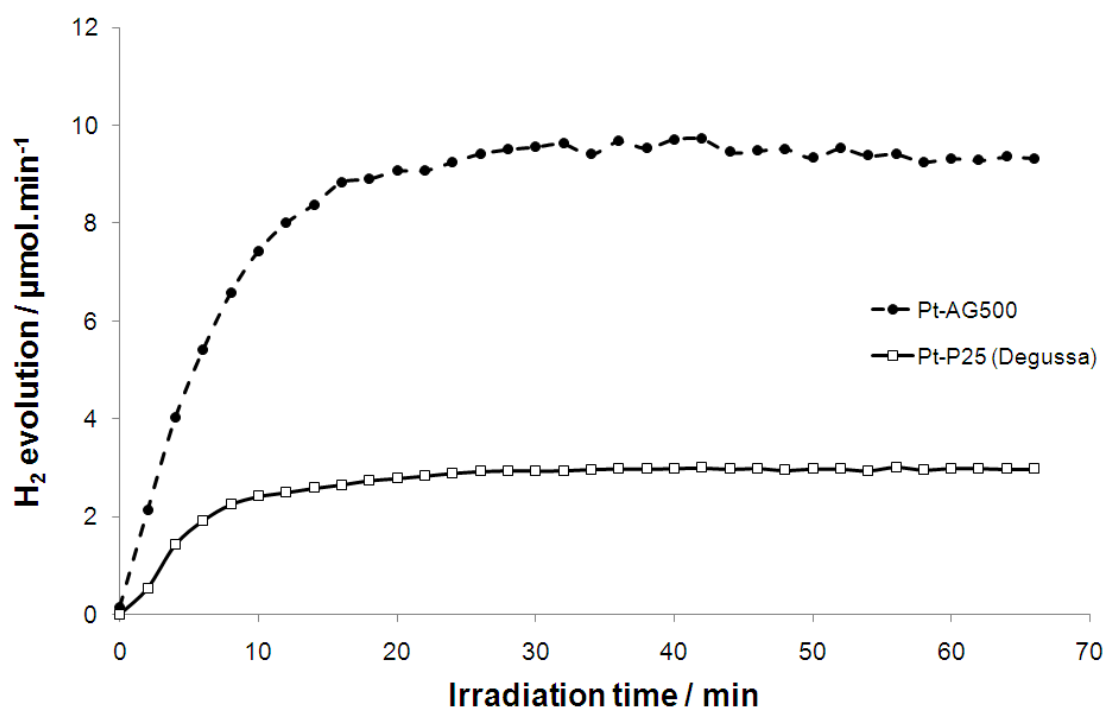
Fig. 19. H 2 evolution on \text{TiO}_2 Pt loaded samples : aerogel calcined at 500 °C and P25 - 150 W metal halide lamp, 0.9 l water + 0.1 l MeOH, 0.7 g samples, 0.3 wt% Pt/ \text{TiO}_2 , room temperature – Strasbourg, France.
