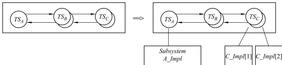
Fig. 10 Partial instantiation of a timed-pNets subsystem
