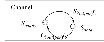
Fig. 8 The timed-pLTS of channel component
