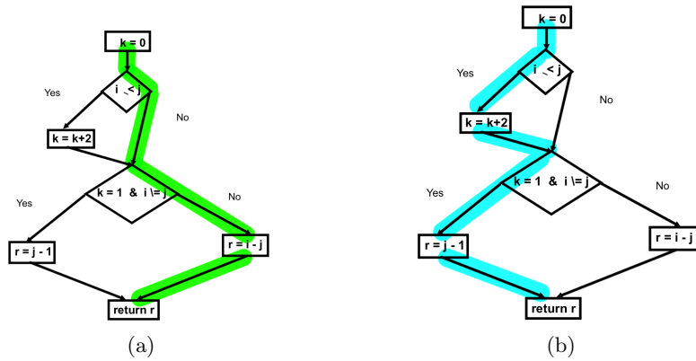
Figure 3: Paths with one deviation – Program AbsMinus
