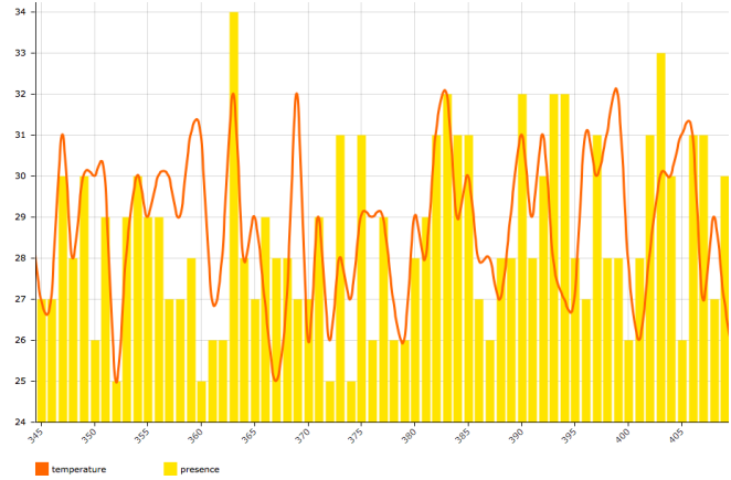
Figure 2. Heating monitoring with temperature and presence correlation.
