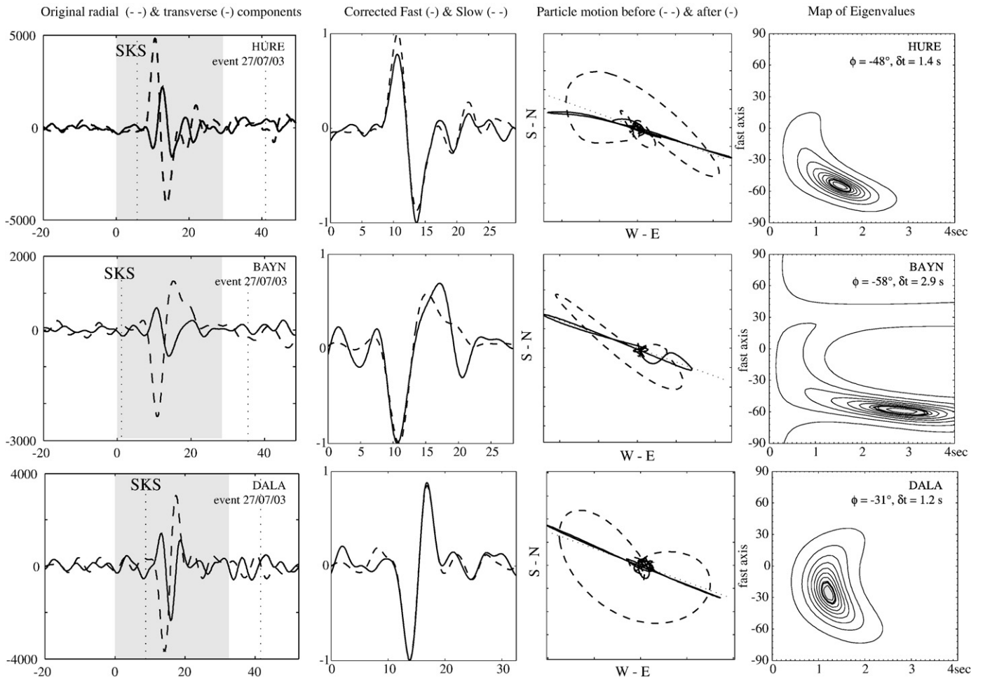
Fig. 2. Examples of splitting measurements obtained for event 2003/208 (27-Jul-2003, 02:04, M_w=6.6 , lat. -21.08^\circ , long. -176.59^\circ , depth 212 km, backazimuth 110^\circ ) at stations HURE, BAYN and DALA. From left to right we show for each station the raw data (radial and transverse components of the SKS phase), the corrected fast and slow split waves, the particle motion in the horizontal plane before and after the anisotropy correction, and the map of the eigenvalues for the various \phi and \delta t values.
