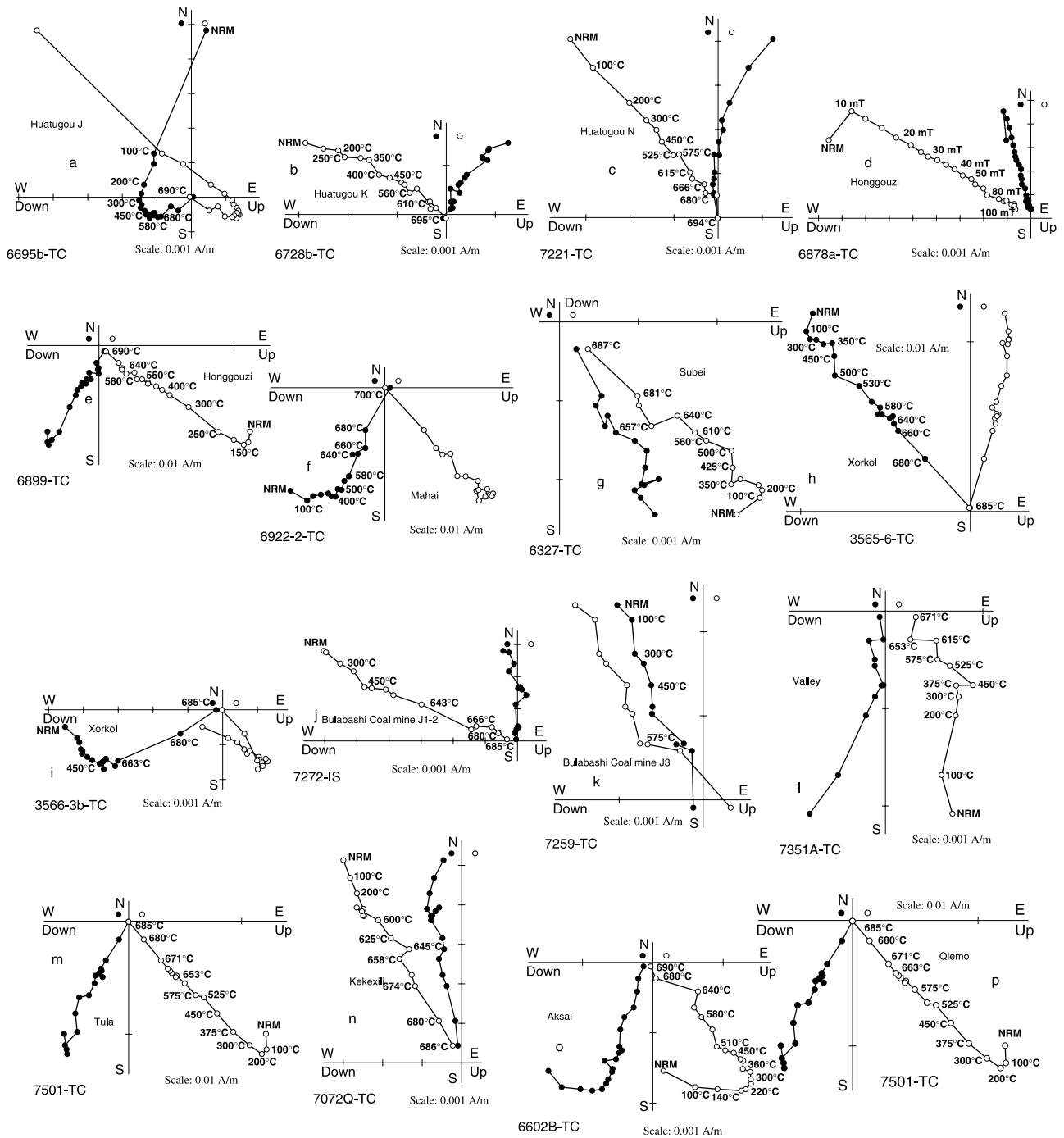
Figure 3. Orthogonal vector plots of representative specimens from each sampled age/locality group. Closed (open) symbols present the projection in horizontal (vertical) plane in stratigraphic coordinates (except 3j).
