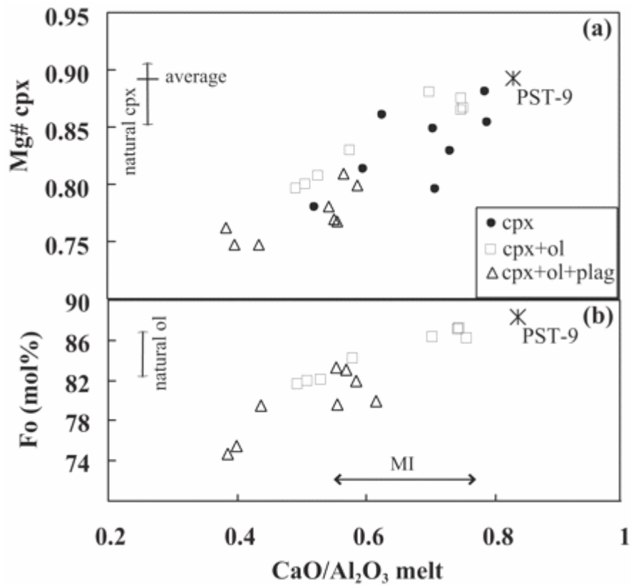
Fig. 6. Mg-number (calculated with FeO t ) in experimental clinopyroxenes (a) and Fo in experimental olivines (b) plotted as a function of the degree of differentiation (CaO/Al 2 O 3 ) of coexisting melts. Data for PST-9 are from Table 1. The range of Mg-number in diopsidic clinopyroxene phenocrysts from golden pumice is shown for comparison (source of data as in Fig. 5), together with the average value. Compositions of homogeneous olivines considered to be in equilibrium with the golden pumices (Fo 83-87 , Bertagnini et al. , 2003) and of their melt inclusions (MI) are also indicated.
