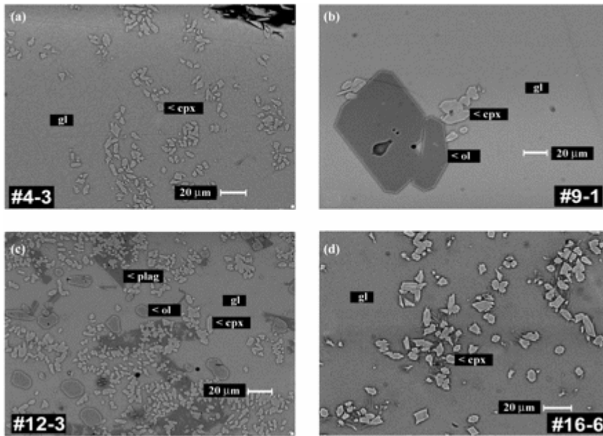
Fig. 2. Backscattered electron images of experimental charges. (See Tables 2 and 3 for experimental conditions.) (a) Typical clinopyroxene crystals in a high-temperature subliquidus charge (4-3). (b) Cotectic crystallization of clinopyroxene + olivine (charge 9-1). The difference in size between the two mineral phases should be noted. (c) Three-phase clinopyroxene + olivine + plagioclase assemblage (charge 12-3) with exceptionally large plagioclase crystals. (d) Illustration of quench crystallization textures with needles of phlogopite(?) nucleating on clinopyroxene (charge 16-6). In contrast, no such phases are present in (a), (b) or (c). gl, glass; cpx, clinopyroxene; ol, olivine; plag, plagioclase.
