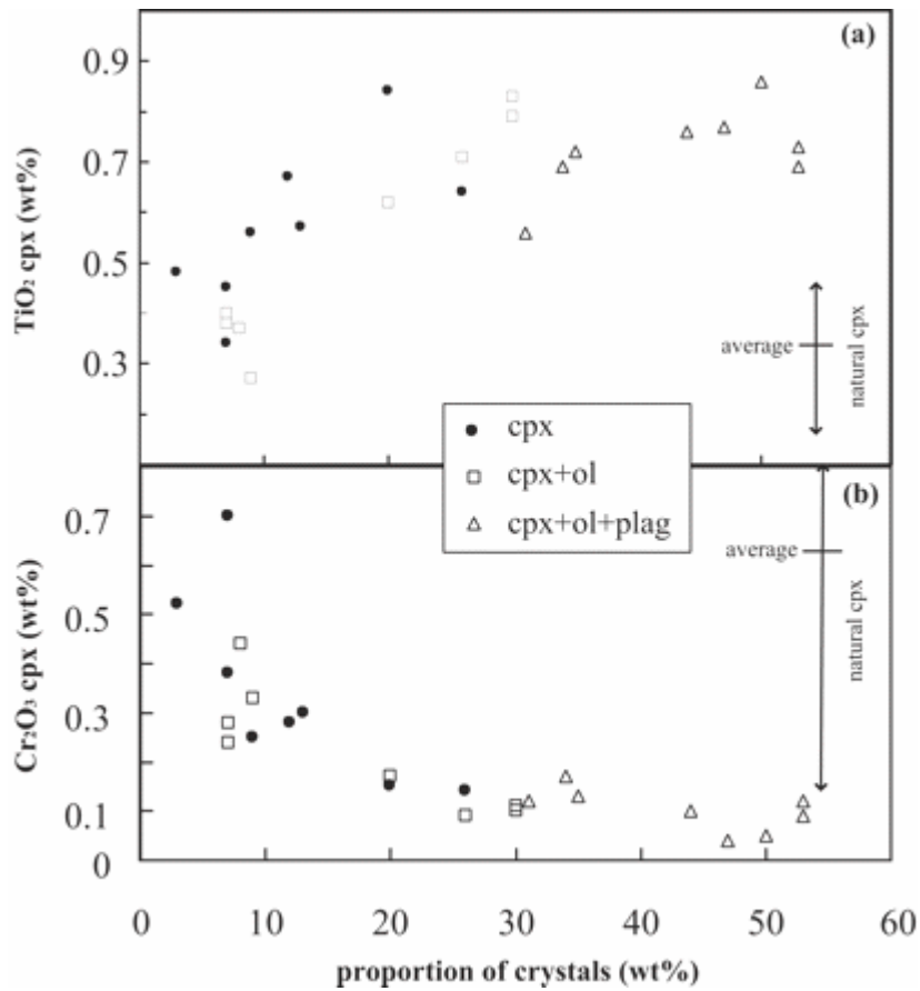
Fig. 5. Dependence of experimental clinopyroxene \text{TiO}_2 (a) and \text{Cr}_2\text{O}_3 (b) contents on the proportion of crystals in the charge (calculated by mass balance; see text). Data are subdivided by phase assemblage (cpx, cpx + ol, cpx + ol + plag). For comparison, the range (i.e. minimum, maximum) of \text{TiO}_2 (a) and \text{Cr}_2\text{O}_3 (b) contents in clinopyroxene phenocrysts and microphenocrysts from golden pumices is shown together with average values. It should be noted that only clinopyroxene compositions from the diopsidic group are compared (source of data: M. Pompilio, unpublished data; Di Carlo, 2004; Francalanci et al. , 2004); that is, the range of clinopyroxene compositions typical of scoriae is not shown
