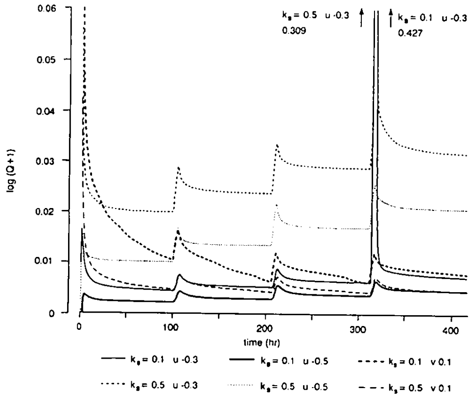
Figure 4.1 Effects of initial pressure potential differences on hillslope discharge: three identical storm events. Q is discharge ( m^3 \text{ hr}^{-1} ) from 1 m slope width; u denotes uniform initial pressure potential at the value (m) indicated; v = 0.1 denotes pressure potential at 0.1 of elevation above datum. (Reproduced, with permission, from Journal of Hydrology , v.130, pp.379-397, 1992).
