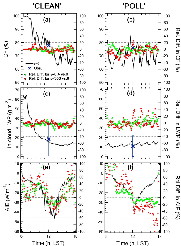
Fig. 1. Time series of cloud fraction (CF, a , b ), in-cloud liquid water path (LWP, c , d ), and aerosol indirect effect (AIE, e , f ) at the top-of-the-atmosphere for the base cases ( \epsilon=0 , black); and the corresponding relative differences (Rel. Diff.) between the base cases and the sensitivity tests ( \epsilon=0.4 , green; \epsilon=300 , red). The left and right panels are for the “CLEAN” (a, c, e) and “POLL” (b, d, f) cases, respectively. The observed values and their uncertainties are indicated with “x” and vertical bars if available.
