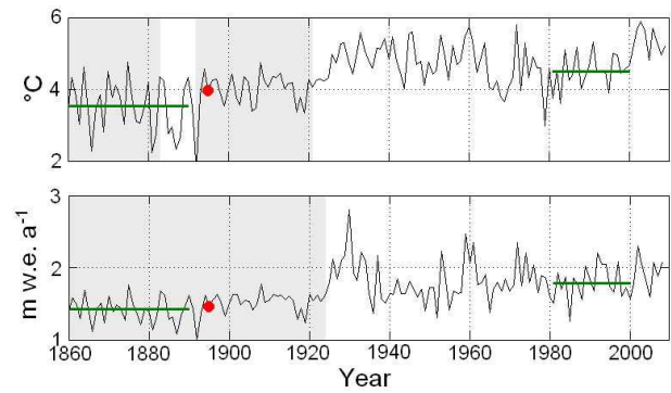
Fig. 8. Mean annual temperature (upper panel) at Hólar in Hornafjörður and precipitation (lower panel) at Fagurhólmýri. The gray areas indicate the periods when the time-series were reconstructed. The horizontal lines indicate the average climate for the two baseline periods 1860–1890 and 1981–2000. The dots show the temperature and precipitation in 1895, the first year of the model simulations.
