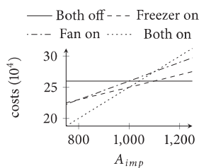
(a) Combined costs of a freezer and a fan as a function of electricity price
