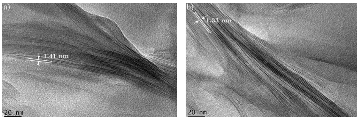
Figure 2: Transmission Electron Microscopy (TEM) images of a) BDTA-Mt organoclay dispersed with 50% ethanol solution and b) C 10 E 3 -Mt organoclay dispersed with 50% ethanol.
