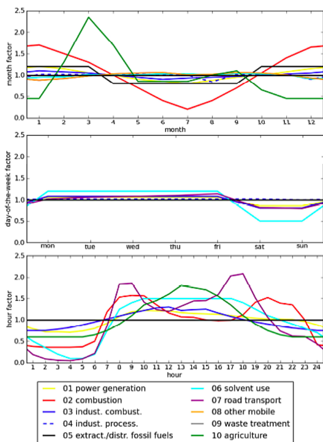
Figure 13. Monthly (top), weekly (middle) and hourly (bottom) time profiles applied to anthropogenic emissions in Europe for different sectors (from Kuenen et al., 2011).
