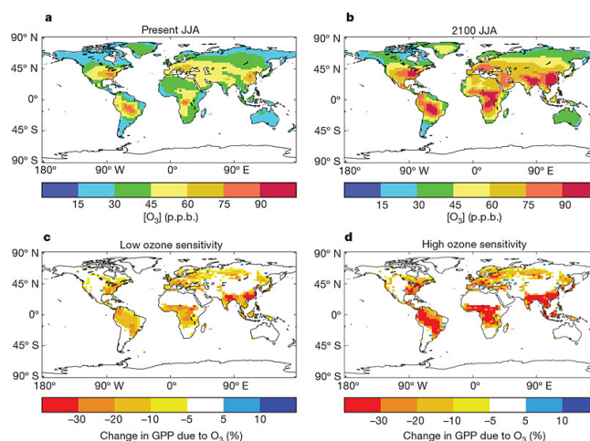
Figure 29. (a, b) Modelled diurnal (24h) mean surface [O 3 ] in ppb averaged over June, July and August (JJA) for the present day (a) and the year 2100 under the highly polluted SRES A2 emissions scenario (b). (c, d) Simulated percentage change in gross primary productivity (GPP) between 1901 and 2100 due to O 3 effects at fixed pre-industrial atmospheric [CO 2 ] for “low” (c) and “high” (d) ozone plant sensitivity (Sitch et al., 2007).
