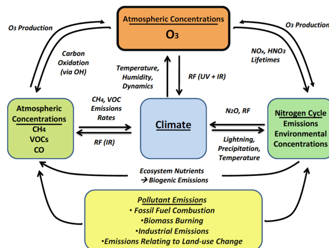
Figure 1. Schematic representation of the interactions of ozone in the Earth system (EPA, 2009).
