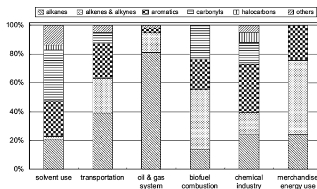
Figure 14. Chemical speciation for various emission sectors in China (Wei et al., 2008) showing the wide variation of VOCs with source that need to be represented in emission inventories.
