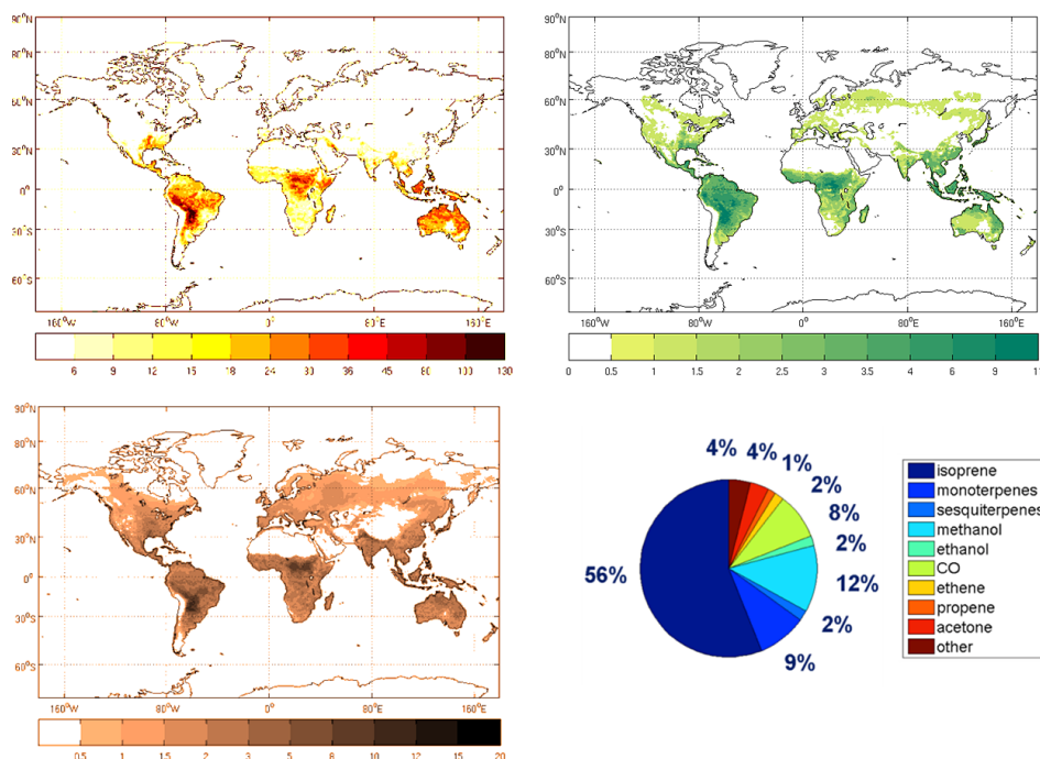
Figure 20. Mean annual emissions (in \text{mg m}^{-2} \text{day}^{-1} ) of isoprene (top left), monoterpenes (top right), methanol (bottom left), and contribution of each BVOCs to the annual global total average (bottom right) (Sindelarova et al., 2014).
