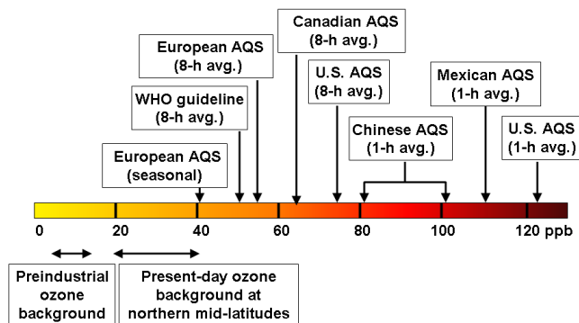
Figure 41. Ozone air quality standards (AQS) in ppb. Different national and international standards are noted as well as estimates for northern mid-latitudes of the pre-industrial background (i.e. O_3 abundances with all anthropogenic emissions of NO_x , CO, VOC, and CH_4 switched off, and before current climate and stratospheric O_3 change) and the present-day baseline abundances (i.e. the statistically defined lowest abundances of O_3 in air flowing into the continents, typical of clean-air, remote marine sites) from Council (2009a).
