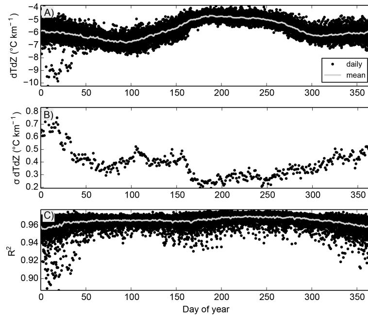
Figure 3. (a) Vertical temperature gradients ( \gamma_T ) by day of year (DOY) for all years (black) calculated from APHRDITE (1961–2007) temperature fields and resampled SRTM data, with period mean in grey, (b) daily standard deviation ( \sigma ) of \gamma_T , and (c) mean daily coefficient of determination ( R^2 ) calculated from the linear regression of resampled SRTM elevations and APHRDITE cell temperatures. All temperature/elevation regressions are significant.
