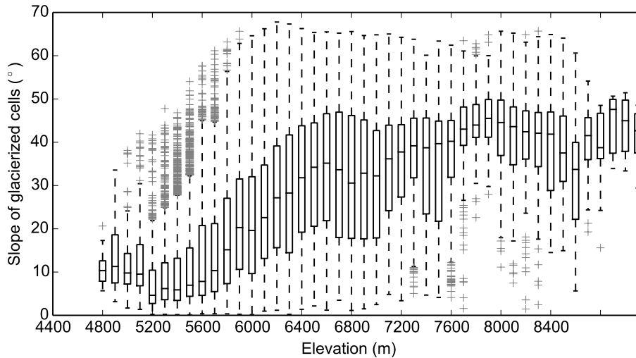
Figure 7. Boxplots of the slope of glacierized pixels in the Dudh Koshi basin, grouped by 100 m elevation bands. The boundaries of each box indicate the upper and lower quartiles, while the middle line of the box shows the median value. Whisker ends indicate the maximum (minimum) values excluding outliers, which are defined as more (less) than 3/2 times the upper (lower) quartile. Slope values were extracted from the SRTM 90 m DEM and glacier inventory from ICIMOD (2011).
