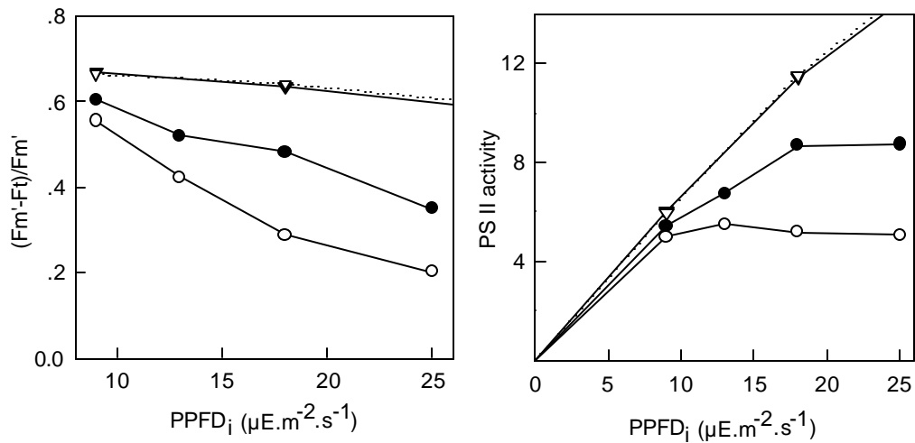
Figure 3. A : PS II quantum yield estimated from (F_m' - F_t) / F_m' as a function of light (incident photosynthetic photon flux density, PPFD i ) in stripped tobacco leaf discs. For anaerobic conditions leaves were flushed with N 2 in the dark during 2 min before light was turned on. Photosynthetic activity was measured 4 min after turning on the light. Anaerobic conditions: control (♦), ndhB - (●); Control and ndhB - under CO 2 -free air (∇;○). B : Photosynthetic flow estimated from (\Delta F / F_m' \times \text{PPFD}_i) as a function of light intensity. Anaerobic conditions: Control (♦); ndhB - (●); Control and ndhB - under CO 2 -free air (∇;○).
