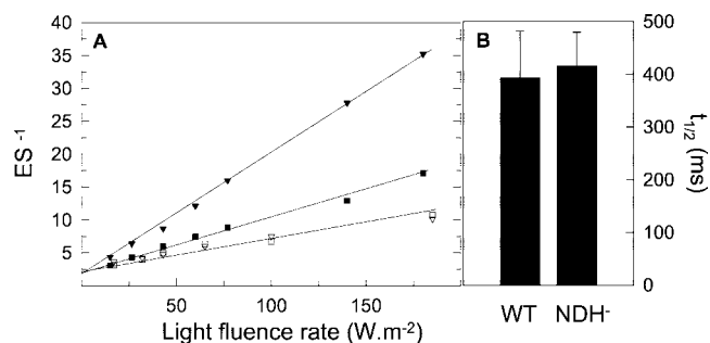
Figure 5. A, Plot of the reciprocal of ES versus the fluence rate of the measuring far-red light ( >715 \text{ nm} ) under anaerobic conditions. ES was measured in WT ( \square , \blacksquare ) and Ndh-less mutant ( \nabla , \blacktriangledown ) at 10 Hz ( \square , \nabla ) and 22 Hz ( \blacksquare , \blacktriangledown ). B, Dark re-reduction of P_{700}^+ after a far-red light period was measured on WT and Ndh-less mutant tobacco leaf discs under anaerobiosis. Data expressing the half-time ( t_{1/2} ) of the P_{700}^+ dark reduction are means \pm SD of 12 experiments.
