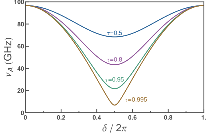
Fig. 5.6. Andreev gap as a function of the phase difference (from Eq. (5.8)), for aluminum single channel contacts of various transmissions, calculated for \Delta = 200 \mu\text{eV} .
