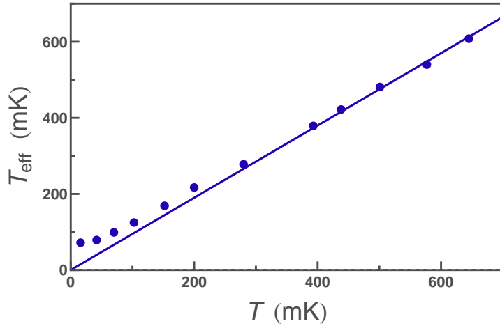
Fig. 4.21. Dots: Effective temperature extracted from switching measurement for various fridge temperatures T . Solid line: the line T_{\text{eff}} = 0.95T , probably accounting for a slight miscalibration of the thermometer. At low fridge temperature, the effective temperature saturates down to 70 mK.
