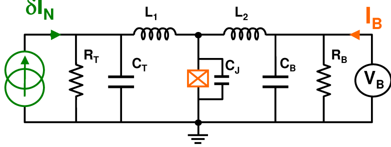
Fig. 4.31. Model circuit designed to capture the behavior of Y^e(\omega) and \alpha(\omega) obtained by microwave simulations in the range [1 – 1.5 GHz] with: R_T = 163\Omega , R_B = 203\Omega , L_1 = 4.9\text{nH} , L_2 = 8.15\text{ nH} , C_T = 0.6\text{ pF} , C_B = 0.85\text{ pF} .
