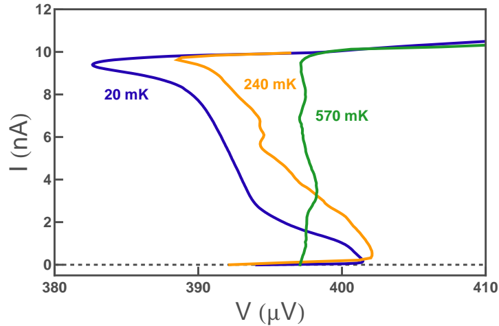
Fig. A.3. Temperature dependence of the back-bending in the noise source of Sample JJD1.
