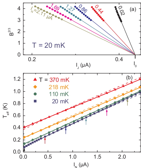
FIG. 2 (color online). (a) Dependence of B^{2/3} = (-\ln(\Gamma/A))^{2/3} on the current I_J through the JJ detector, for data taken at T = 20 mK and currents through the tunnel junction I_N = 0.02 to 2.11 \mu\text{A} , by steps of 0.42 \mu\text{A} . Linear dependence is a signature of the thermal activation regime. (b) Effective temperature extracted from the slope of data sets as in (a), as a function I_N , for various temperatures T . Arrows indicate the data points corresponding to the plots in (a). Solid lines are linear interpolations. Dashed lines are the predictions from full theory, taking into account the frequency dependence of the admittance Y(\omega) across the JJ and of the transfer function \alpha(\omega) from noise source to JJ detector.
