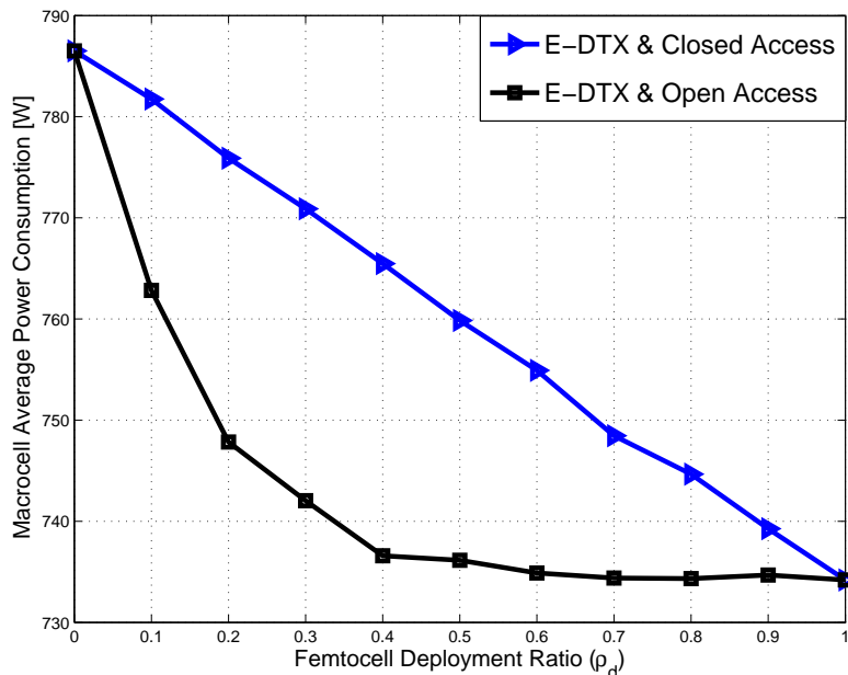
Figure 5.5: Macrocell average Power Consumption with respect to the femtocell deployment ratio ( \rho_d ).
