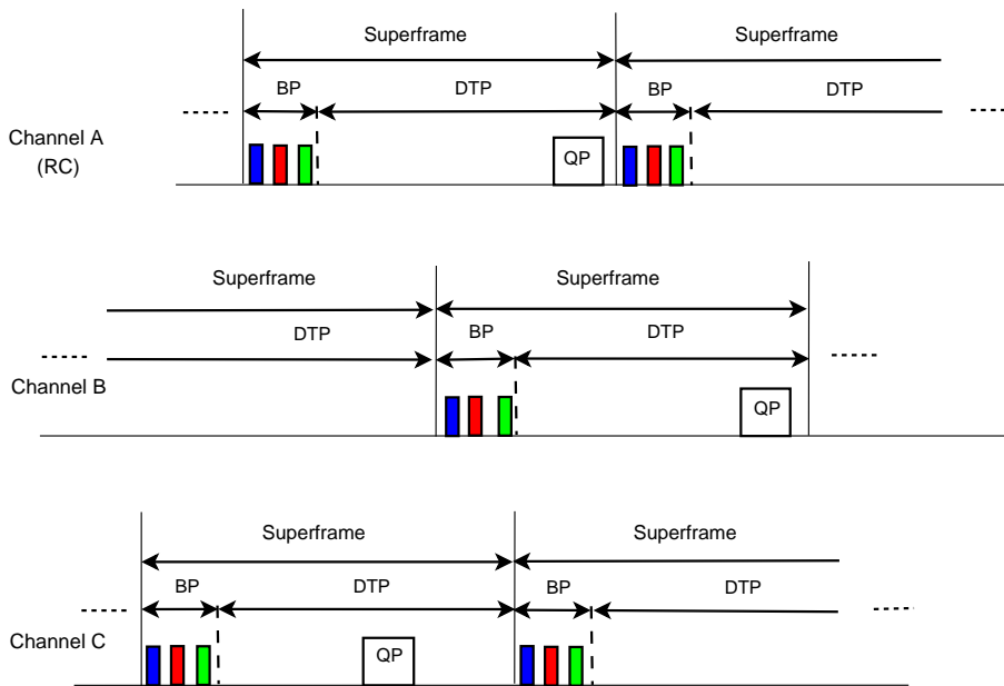
Figure 2.20: Channel superframe structure in C-MAC [53].
