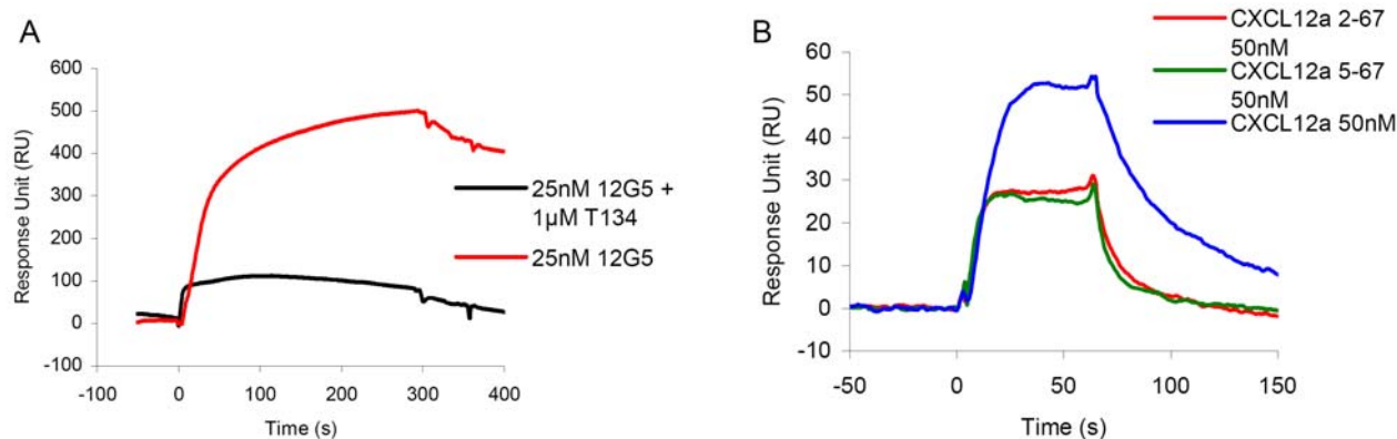
Figure 5.5 (A) 25nM 12G5 binding to immobilized CXCR4 in the absence (red curve) and presence (black curve) of 1 \mu M T134 antagonist. (B) Native CXCL12 \alpha (50nM, blue curve), mutant CXCL12 \alpha 2-67 (red curve) and mutant CXCL12 \alpha 5-67 (green curve) binding to immobilized CXCR4.
