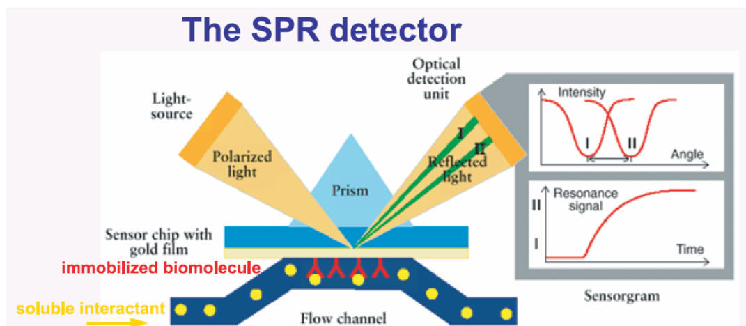
Figure 8.5 Binding is measured as a change in the refractive index as the sensor surface. A change of 0.001 degrees is equivalent to 1pg of protein bound per mm 2 .
