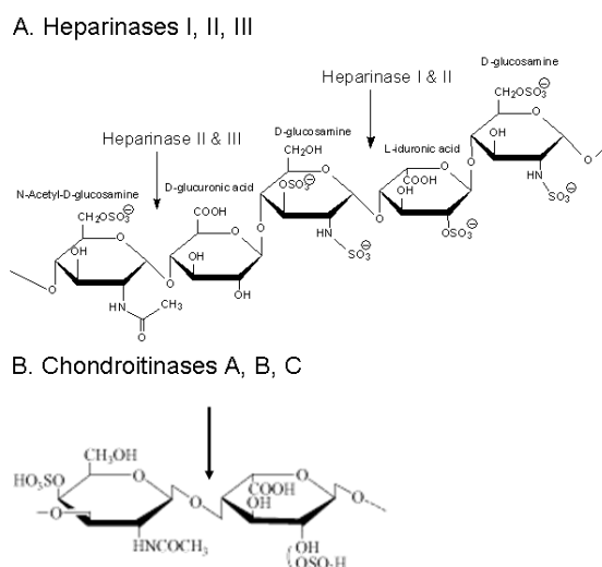
Figure 2.4 (A) The heparinases cut the oligosaccharide at the \alpha 1-4 glycosidic liaison between a glucosamine and a uronic acid (GlcA or IdoA). Heparinase I cuts between a hexosamine and a 2- O -sulphated uronic acid. Heparinase II cuts between a hexosamine and a uronic acid and heparinase III cuts between a hexosamine and a glucuronic acid. (B) Chondroitinase ABC cut between the N-acetyl hexosamine and the uronic acid.
