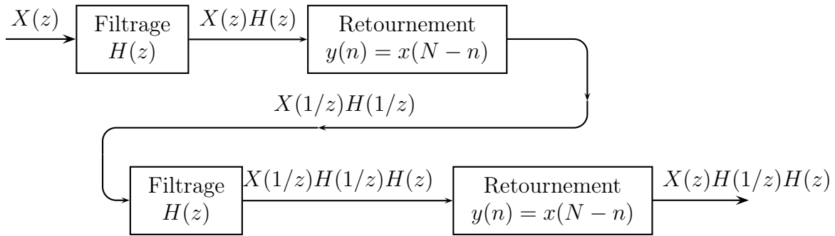
FIGURE 3.5: Principe du filtrage "forward-backward"
