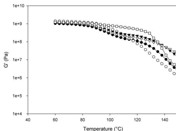
Figure 41 : Storage modulus G' comparison in the region of the ionic plateau PS(x) ( CaCO_3/MAA = x ); \square PS(0.0) , \bullet PS(0.7) , \circ PS(0.8) , \blacktriangledown PS(1.2) , \nabla PS(1.4)
