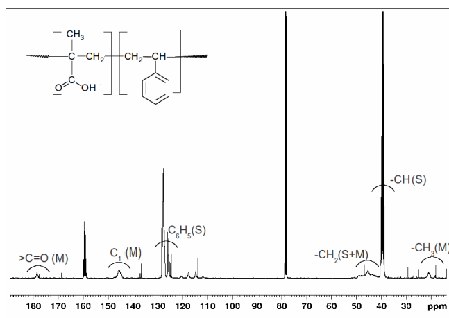
Figure 31 : ^{13}\text{C} -NMR spectra of the 50S50MAA copolymer in DMSO- d_6 and \text{CDCl}_3 (50/50 volume%) with TFA at 20°C
