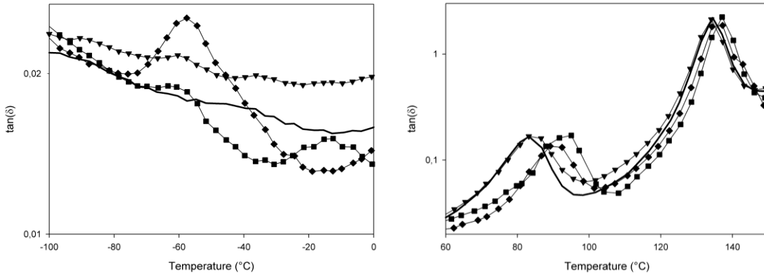
Figure 77 : \tan\delta vs temperature in the solid state of blends extruded at 220°C and 200rpm : - PC+PS (70/30 wt%) without copolymer; ▲ PC+PS(70/30 wt%)+1.125 wt % SEBS-g-PC ; ■ PC+PS(70/30 wt%)+2.5wt% SEBS-g-PC ; ◆ PC+PS(70/30 wt%)+5wt% SEBS-g-PC
