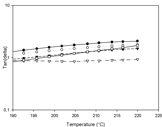
Figure 42 : Tan(\delta) in the melt state for each copolymer PS(x) ( CaCO_3/MAA = x ); \square PS(0.0) , \bullet PS(0.7) , \circ PS(0.8) , \blacktriangledown PS(1.2) , \nabla PS(1.4)
