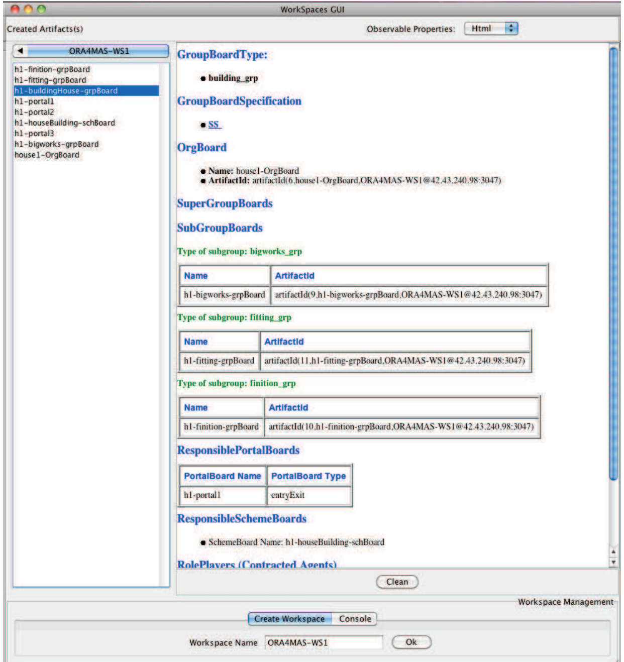
FIGURE E.2 – GroupBoard building_grp : h1-buildingHouse-grpBoard
