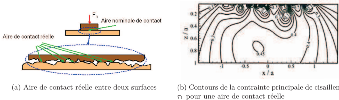
FIGURE 1.19 : Contact réel (Hutchings, 1992)
