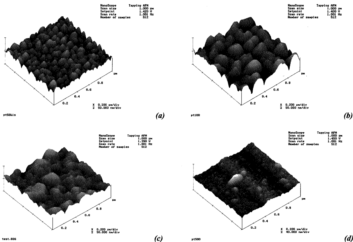
Figure III.8. : surface d'une couche de platine de 50 Å (a), 100 Å (b), 200 Å (c) et 500 Å (d).
