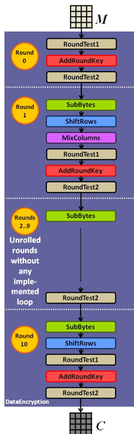
Figure 5.6: Implementation of the unrolled AES with RoundTest1 and RoundTest2 operations.
