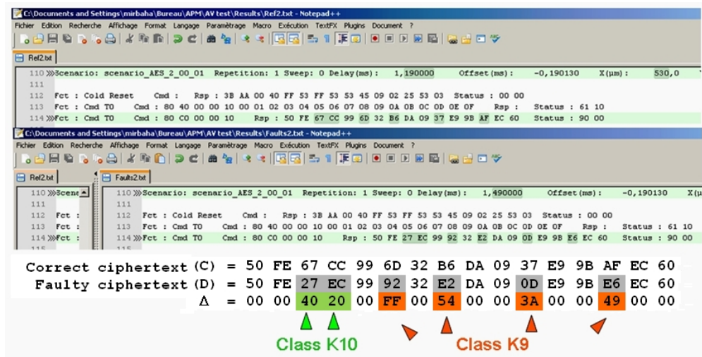
Figure 3.15: Classification of faulty bytes on the ciphertext. Faults are separated into two classes of corresponding ( K_9 -related) and non-corresponding ( K_{10} -related) faults for Giraud’s bit DFA.
