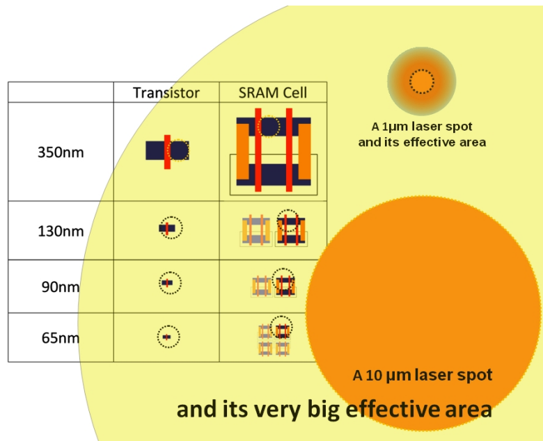
Figure 3.1: 1 µm & 10 µm laser spot diameters vs technology scaling.
