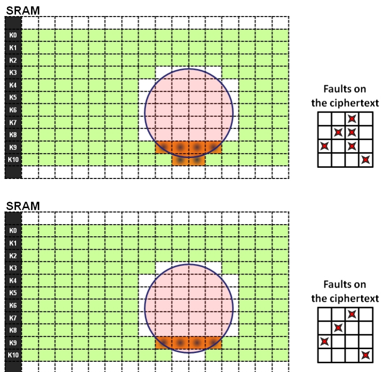
Figure 3.14: Exploration process and results classification. The laser emission time is set to t_9 during exploration. Then, the classification process excludes K_{10} -related faults.
