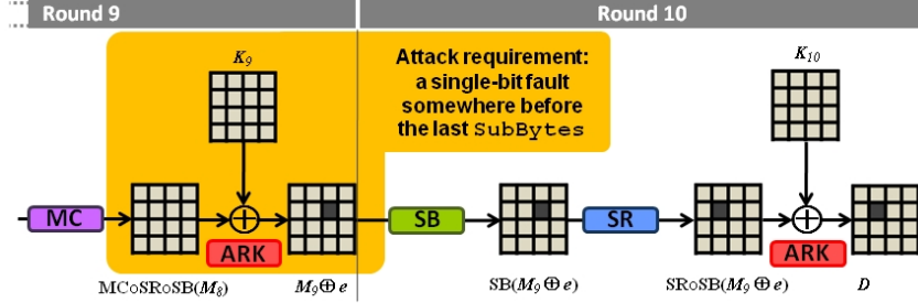
Figure 3.8: Giraud’s bit DFA.
