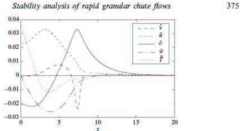
FIGURE 7. Real part of the eigenfunctions ( \hat{v}(z) , \hat{u}(z) , \hat{\phi}(z) , \hat{w}(z) , \hat{T}(z) ) corresponding to the stationary mode ( h = 8 , \bar{v} = 0.23 , k = 0.4 , e = 0.6 , \phi = 0.05 ).
