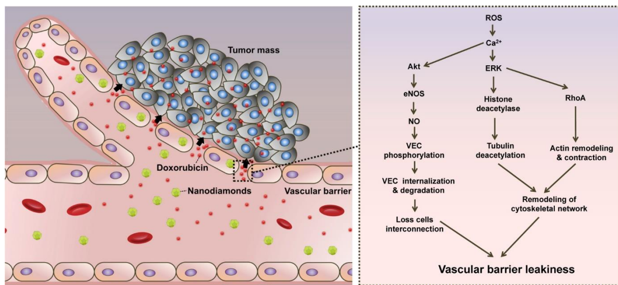
Fig. 11 Schematic representation of nanodiamond (ND)-induced vascular barrier leakiness. ND-induced vascular barrier leakiness leads to higher accumulation of doxorubicin in the tumor site. The increase of intracellular ROS and \text{Ca}^{2+} account for the ND-induced vascular barrier leakiness through the loss of cell-cell interconnection in the vascular barrier and cytoskeletal remodeling. Reproduced with permission from ref 310
