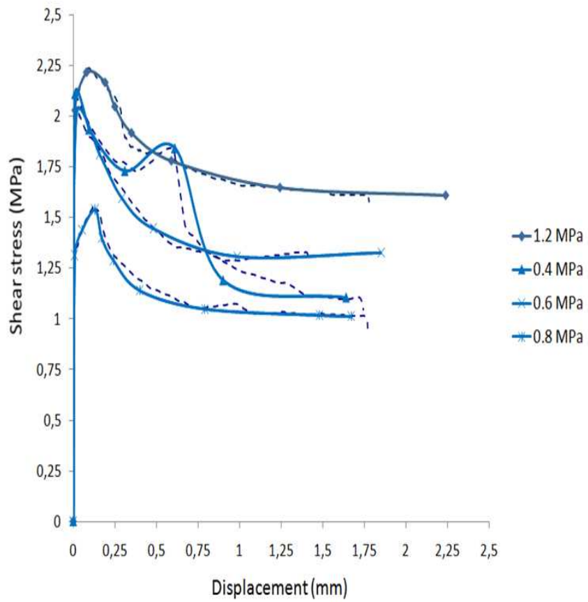
Figure 18: Effect of the confining pressure: Experimental and numerical "shear stress-displacement" diagrams of a small confined wall under shear loading conditions.
